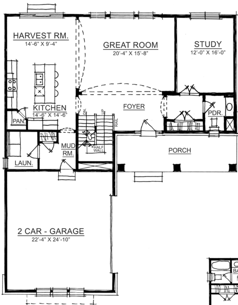
Main Level
