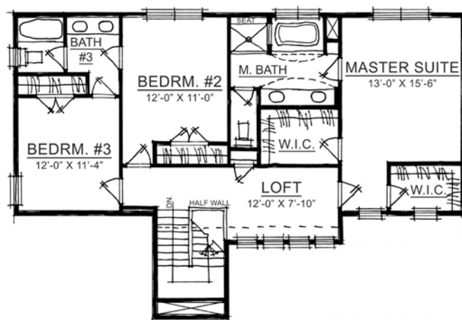
Upper Level
