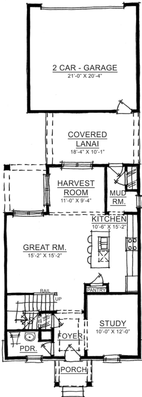
Main Level
