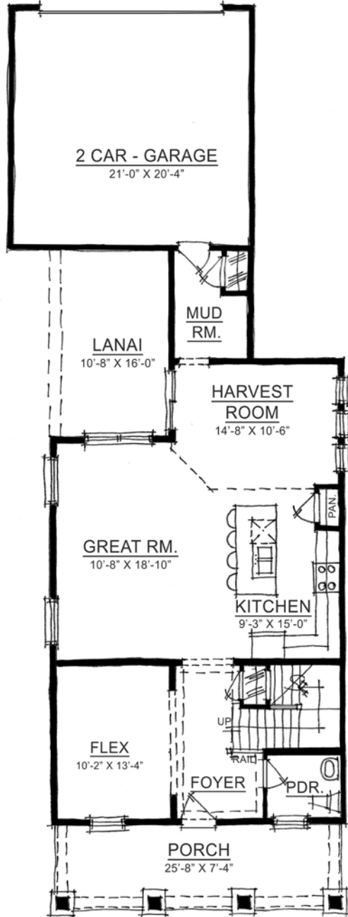
Main Level
