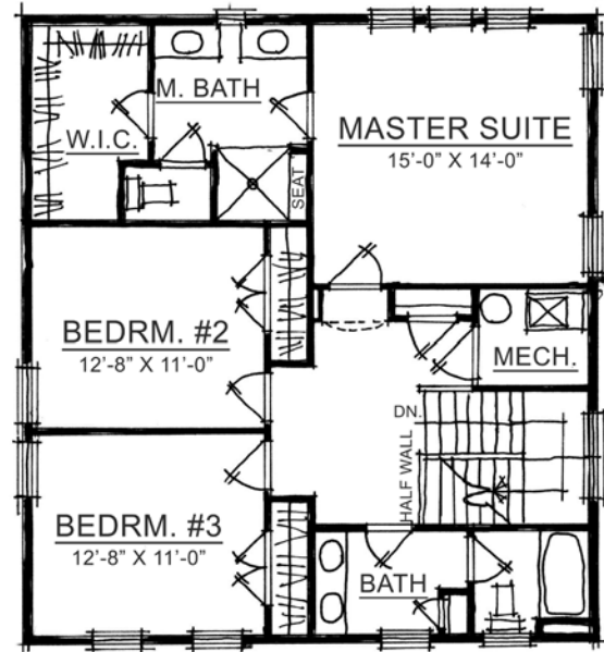
Upper Level
