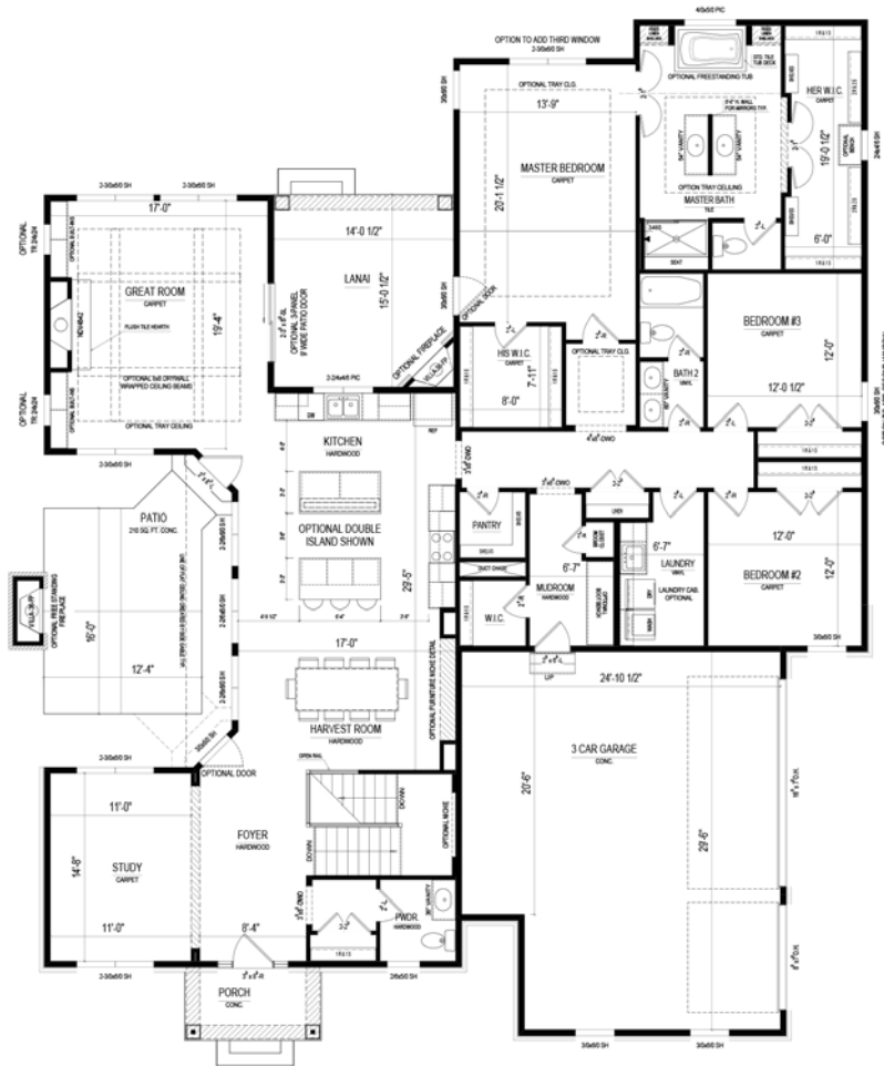
Main Level
