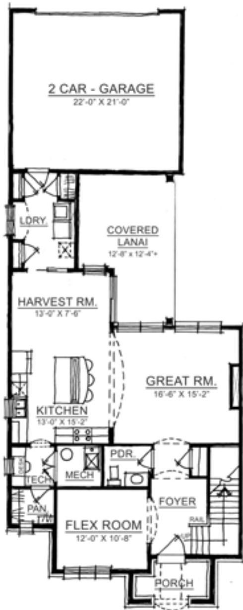
Main Level
